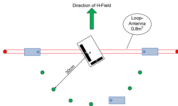
Figure 5: Antenna Direction - vertical to X-Y-Plane of the avalanche transceiver.
